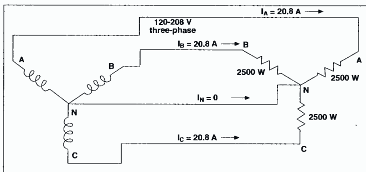
Figure 2. A wye-connected source and load using a neutral wire. The neutral wire carries current that results from any imbalance in the loads.
