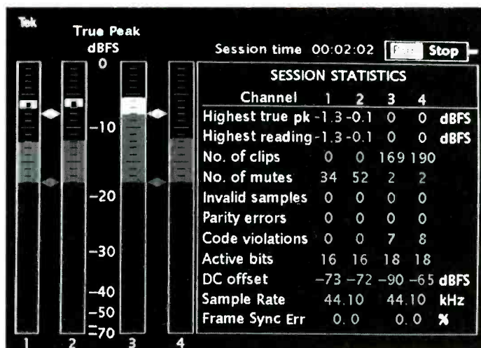
Figure 2. Signal characteristics are accumulated and displayed on the session screen, along with continuing indications of signal level.
