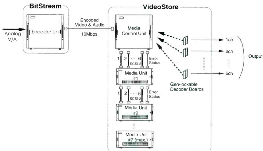
Figure 1. Basic setup of the BitStream and VideoStore units for multiple channel outputs. Each Media Unit provides a storage capacity of 4.5 hours.
