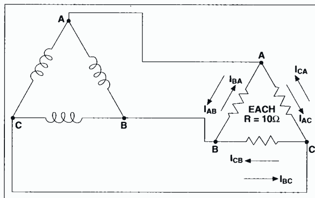
Figure 1. A balanced load connected to a delta supply in a delta configuration.
