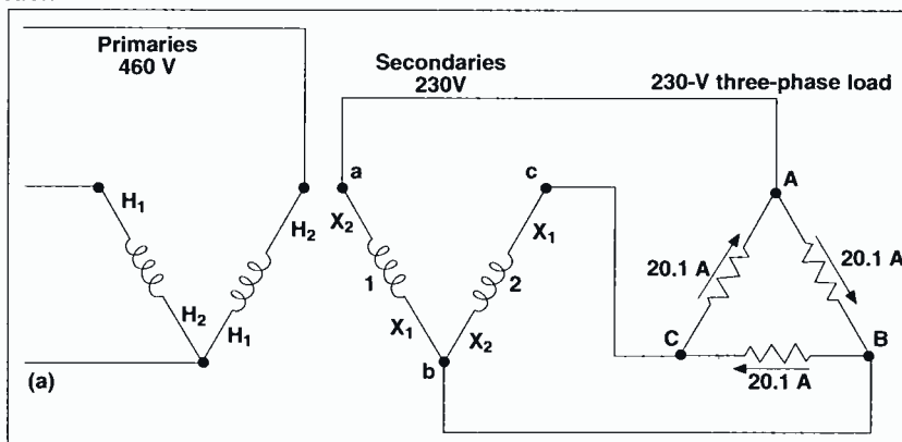
Figure 3. Transformers connected in open-delta system supplying a balanced 3-phase resistive load. This arrangement is not recommended for use in broadcast transmitters.
